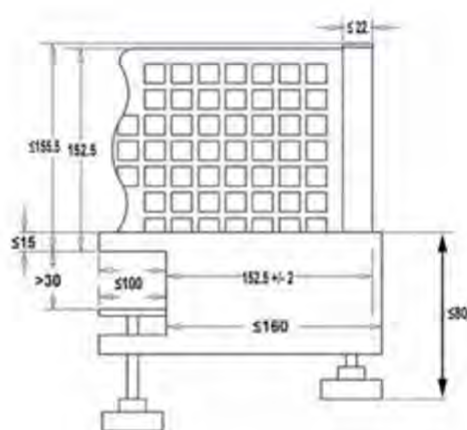
Figure 2: Front view
