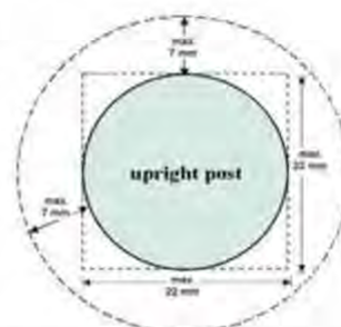
Figure 4: Cut through upright post
